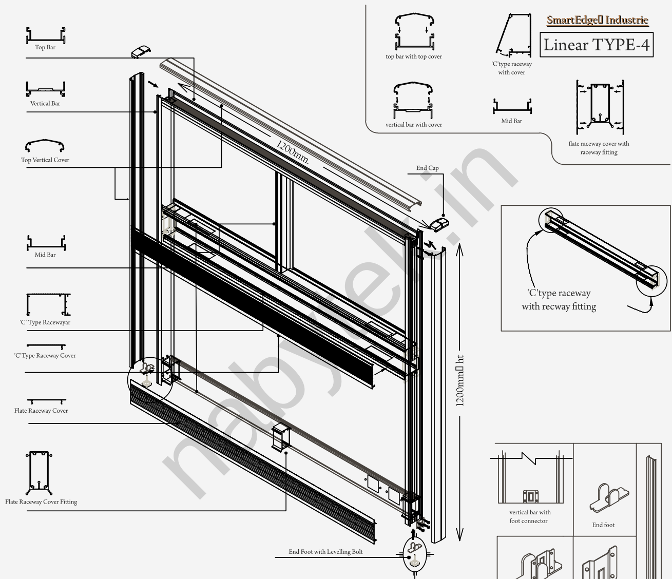
Linear 60mm.Panel Based Double Raceway Below top & Skirting Level.
